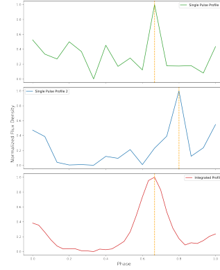
(b) Single-pulse detections from PSR J0248+4230 in uGMRT Band-3. The top and middle panels show two individual bright single-pulse profiles, while the bottom panel shows the integrated profile. The first single pulse peaks at phase 0.67, aligned with the integrated profile, whereas the second bright pulse peaks at phase 0.80, offset from the average peak.
